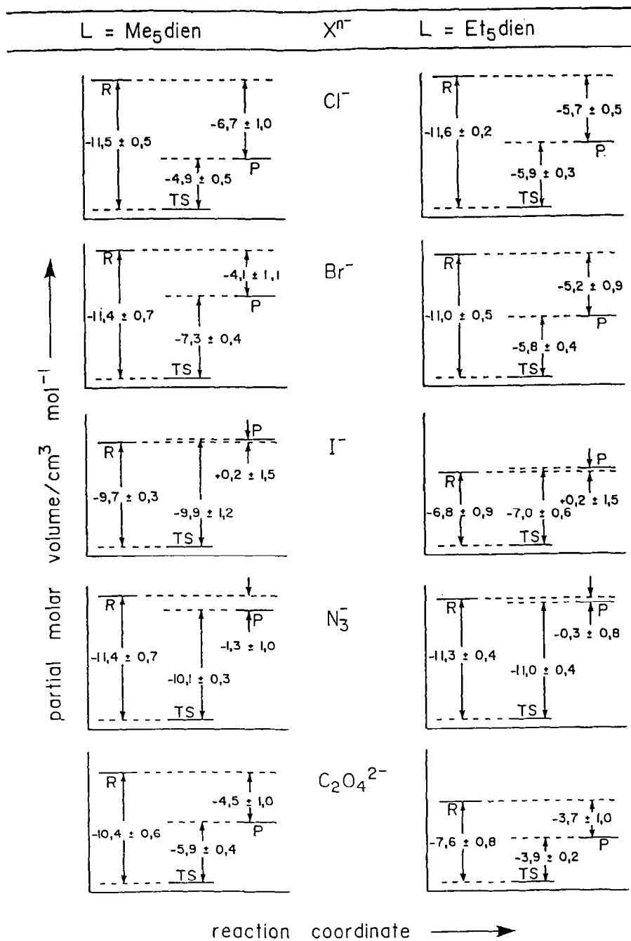
Fig. 4. Volume profiles for the reaction [38]: Pd(L)X (2-n)+ + H 2 O ⇌ Pd(L)H 2 O 2+ + X n- .
