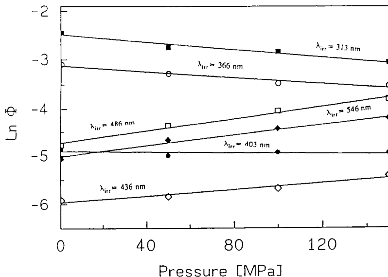
Fig. 11. Plot of natural logarithm of the quantum yield versus pressure at different excitation wavelengths for the reaction [84]: M(CO)_4(phen) + PR_3 \rightarrow fac-M(CO)_3(PR_3)(phen) + CO ; ( M = Mo , R = Bu^t ).
