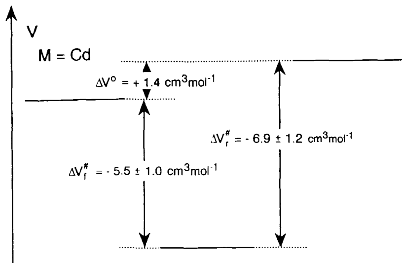
Fig. 2. Volume profiles for formation and dissociation of M(H_2O)_4(bpy)^{2+} complexes; M = Zn, Cd [16,17].
