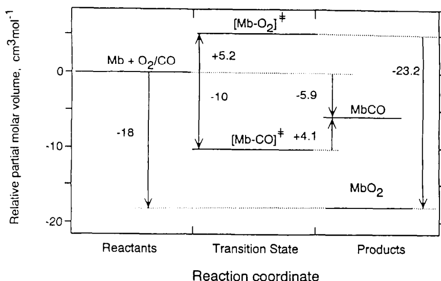
Fig. 16. Volume profile for the reactions of \text{CO} and \text{O}_2 with myoglobin at 298 K [131].
