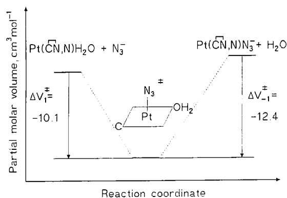
Fig. 9. Volume profile for anation of \text{Pt}(\text{C}-\text{N}, \text{N})\text{H}_2\text{O}^+ by azide [59].
