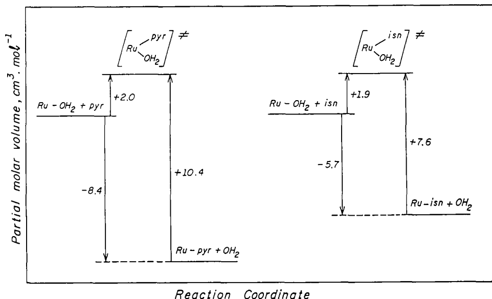
Fig. 7. Volume profiles for the reaction [54]: \text{trans} - [\text{Ru}(\text{NH}_3)_4\{\text{P}(\text{OEt})_3\}(\text{H}_2\text{O})]^{2+} + \text{L} \rightleftharpoons \text{trans} - [\text{Ru}(\text{NH}_3)_4\{\text{P}(\text{OEt})_3\}\text{L}]^{2+} + \text{H}_2\text{O} , where L = pyrazine (left) or isonicotinamide (right). The metal complexes are shown in abbreviated forms.
