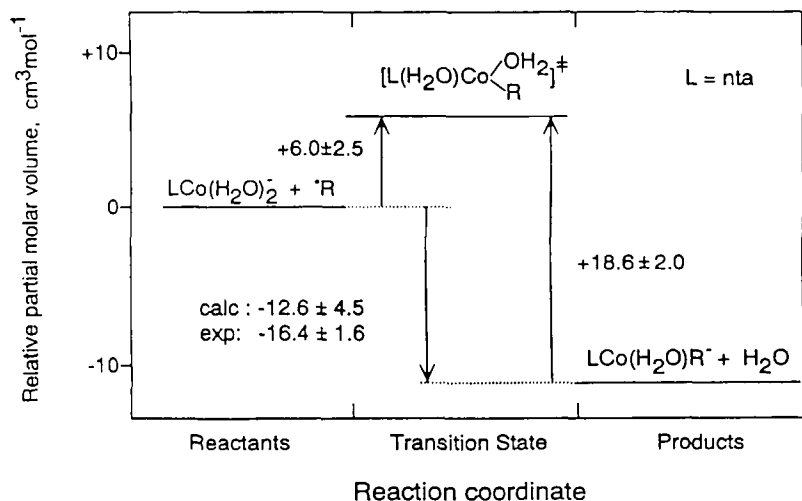
Fig. 12. Volume profile for the reaction of methyl radicals with the nitrilotriacetate complex of Co(II) at 298 K [93].
